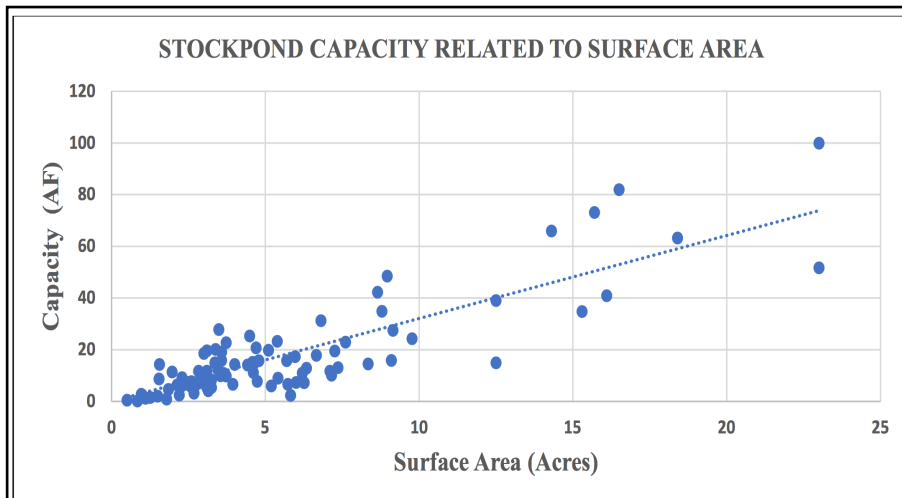
Figure 3. Data plotted for stockponds measured in the field shows the relationship between capacity and surface area. The dotted line results from regression analysis of the data. Source. Technical Report, Figure 4-5
